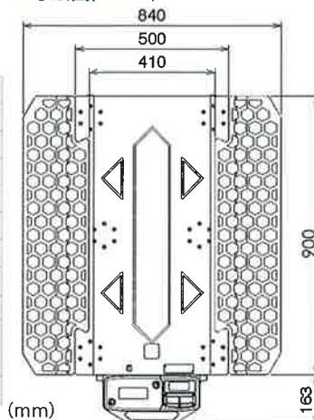
■寸法図(900mm)
